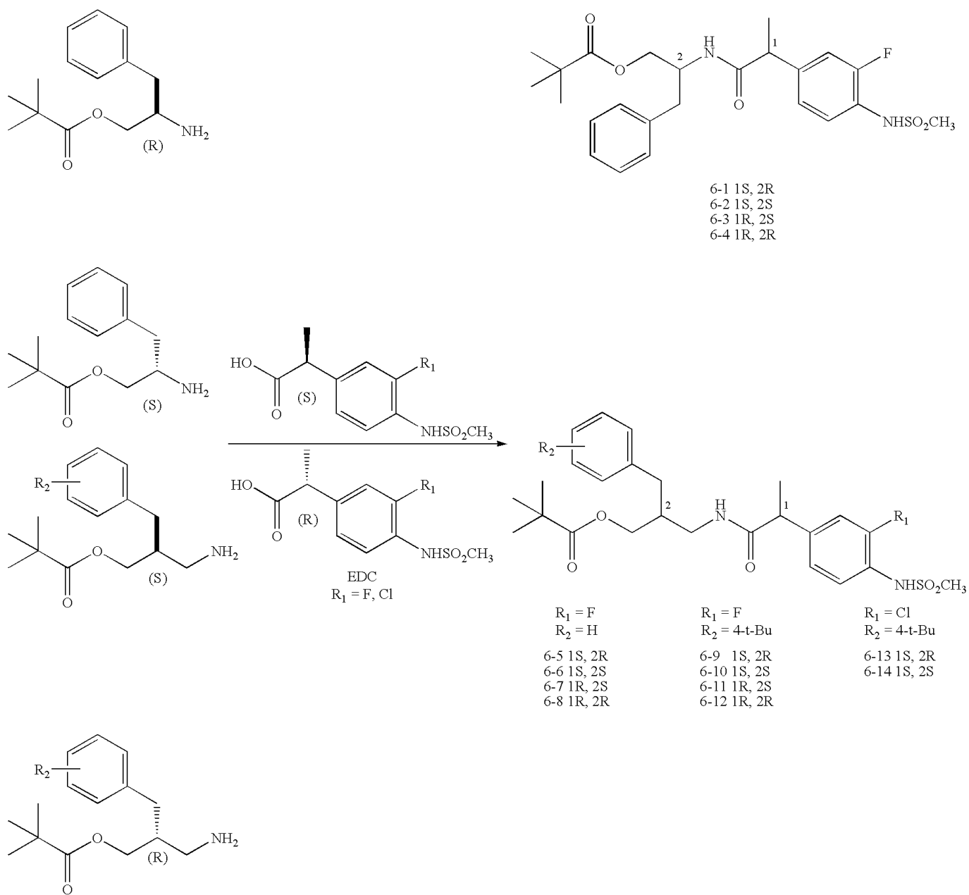
Scheme 6
